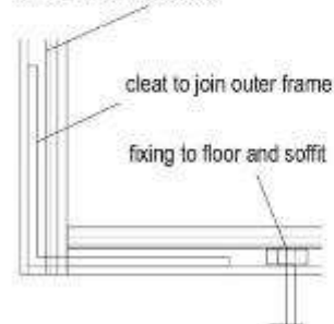
GP-18100D assembly of components and fixing
