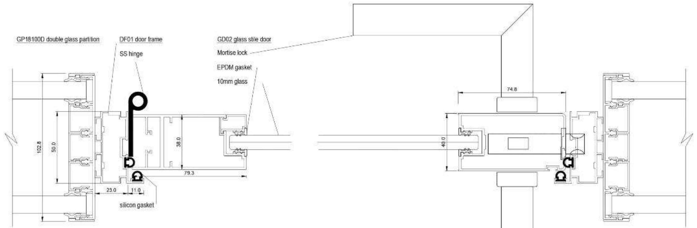
Assembly of Glass partition GP-18100D with Door frame DF01 and glass door GD02
