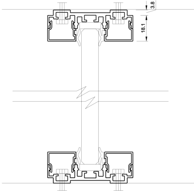
GP-2160S assembly of components and fixing
