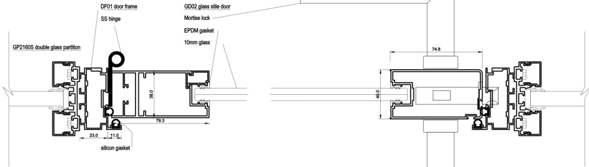
Assembly of Glass partition GP-2160S with Door frame DF01 and glass door GD02
