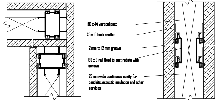
CORNER DETAIL WPD3P PLAN
